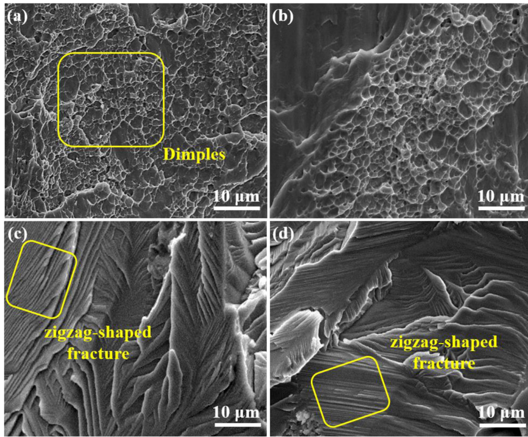
Fig. 3. Fracture surfaces of the \text{Al}_2\text{O}_3 -reinforced alloys compressed at room temperature (a) HfNbTaTiZrV alloy, (b) 1 vol.% \text{Al}_2\text{O}_3 alloy, (c) 2 vol.% \text{Al}_2\text{O}_3 alloy, (d) 4 vol.% \text{Al}_2\text{O}_3 alloy.
