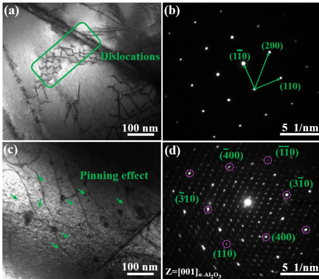
Fig. 7. Bright-field TEM images of alloy with 5% strain at room temperature (a) HfNbTaTiZrV alloy, (b) SAED pattern of (a), (c) 4 vol.% Al 2 O 3 alloy, (d) SAED pattern of (c).
