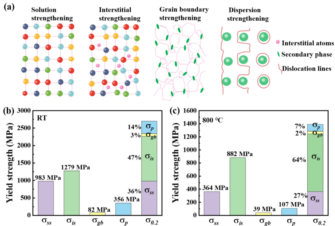
Fig. 10. (a) Schematic diagram of the solid strengthening, interstitial strengthening, grain boundary strengthening, and dispersion strengthening, respectively. Contributions of different strengthening mechanisms in the 4 vol.% Al 2 O 3 alloy during compression at (b) Room temperature and (c) 800 °C.
