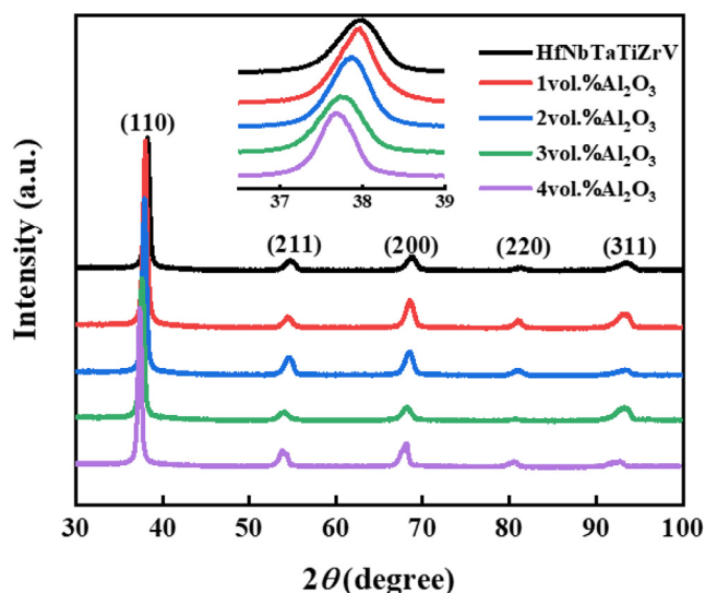
Fig. 1. XRD patterns of the as-cast x vol.% Al_2O_3 -reinforced HfNbTaTiZrV alloys at room temperature.
