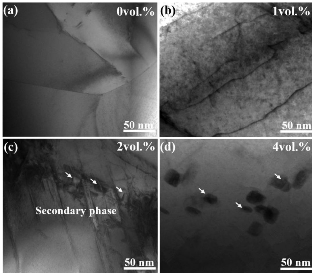
Fig. 5. Bright-field TEM images as-cast \text{Al}_2\text{O}_3 -reinforced alloys (a) HfNbTaTiZrV alloy, (b) 1 vol.% \text{Al}_2\text{O}_3 alloy, (c) 2 vol.% \text{Al}_2\text{O}_3 alloy, (d) 4 vol.% \text{Al}_2\text{O}_3 alloy.
