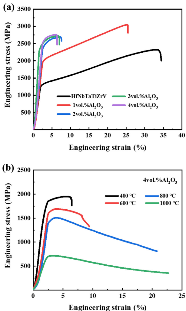
Fig. 2. Compressive engineering stress-strain curves of (a) the as-cast 0–4 vol.% \text{Al}_2\text{O}_3 -reinforced HfNbTaTiZrV alloys at room temperature, (b) 4 vol.% \text{Al}_2\text{O}_3 alloy at elevated temperatures.
