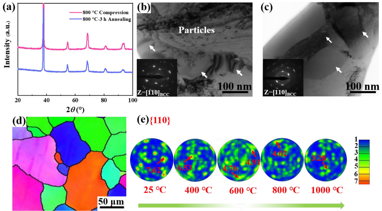
Fig. 9. Microstructure of the 4 vol.% Al 2 O 3 alloy (a) X-ray diffraction patterns of various treatment, (b) Bright-field TEM image of the 4 vol.% Al 2 O 3 alloy after 800 °C compression, (c) Bright-field TEM image of the 4 vol.% Al 2 O 3 alloy after annealing at 800 °C for 3 h, (d) EBSD image of the 4 vol.% Al 2 O 3 alloy after 800 °C compression, (e) Pole figures for {110} BCC of the 4 vol.% Al 2 O 3 alloy deformed at various temperatures.
