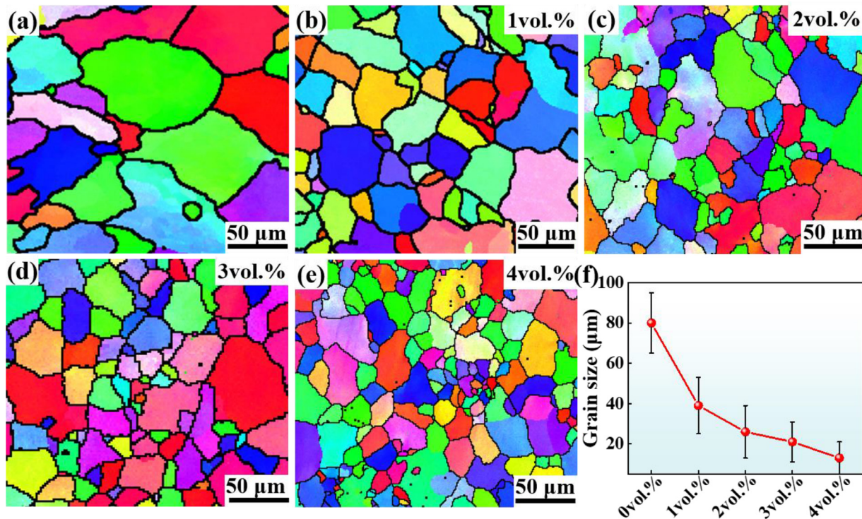
Fig. 4. EBSD images of the as-cast \text{Al}_2\text{O}_3 -reinforced HfNbTaTiZrV alloys at room temperature (a) HfNbTaTiZrV alloy, (b) 1 vol.% \text{Al}_2\text{O}_3 alloy, (c) 2 vol.% \text{Al}_2\text{O}_3 alloy, (d) 3 vol.% \text{Al}_2\text{O}_3 alloy, (e) 4 vol.% \text{Al}_2\text{O}_3 alloy, (f) Average grain size of the alloys.
