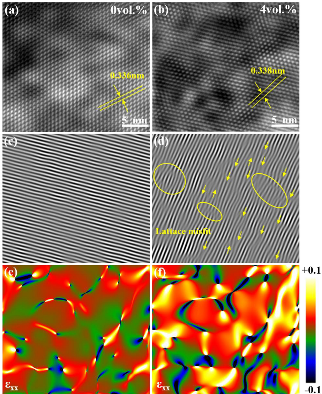
Fig. 8. Lattice uniformity analysis of the HfNbTaTiZrV and 4 vol.% Al 2 O 3 alloy alloys (a) and (b) HRTEM images of the HfNbTaTiV and 4 vol.% Al 2 O 3 alloys viewed in [110] direction, respectively. (c) and (d) Inversed FFT images of (a) and (b), respectively. (e) and (f) Distribution maps of interatomic distances along [121] in the HfNbTaTiZrV and 4 vol.% Al 2 O 3 alloys, respectively.
