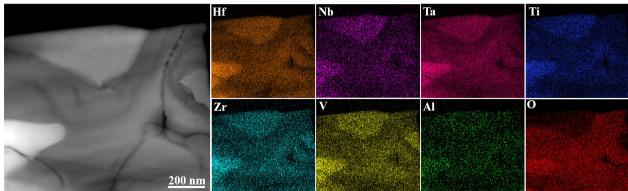
Fig. 6. HAADF-STEM micrograph of the as-cast 4 vol.% \text{Al}_2\text{O}_3 alloy along the [110] zone axis ( Im\bar{3}m ) and EDS mappings showing the distribution of elements.
