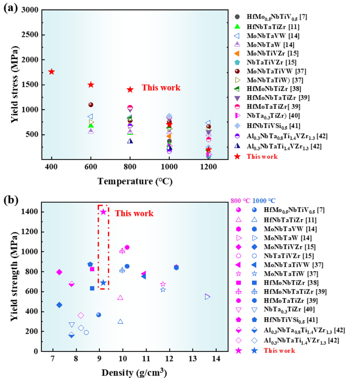
Fig. 11. Mechanical property comparison between the 4 vol.% Al 2 O 3 alloy and other RHEAs (a) Temperature dependence on the yield strength, (b) Density-yield strength at elevated temperatures of 800 and 1000 °C.
